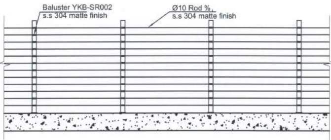
Railing Elevation 护栏立面图
