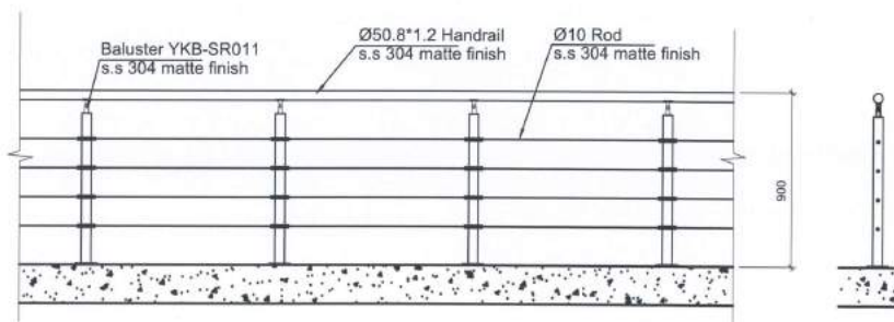
Railing Elevation 护栏立面图
