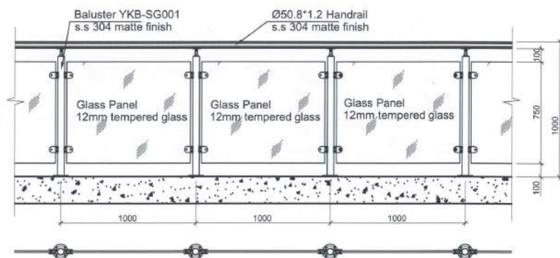
Railing Elevation 护栏立面图
