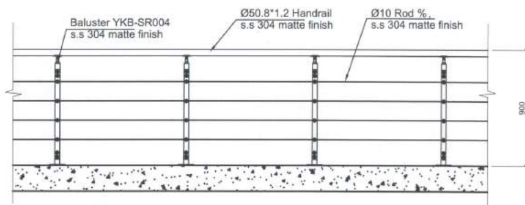
Railing Elevation 护栏立面图
