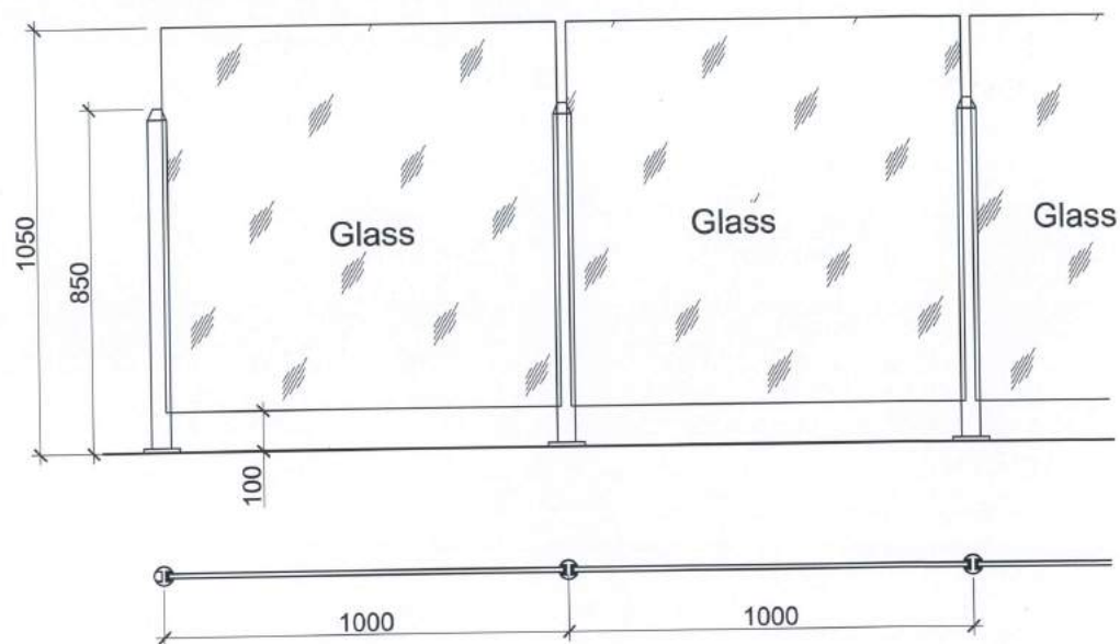
Railing Elevation 护栏立面图
