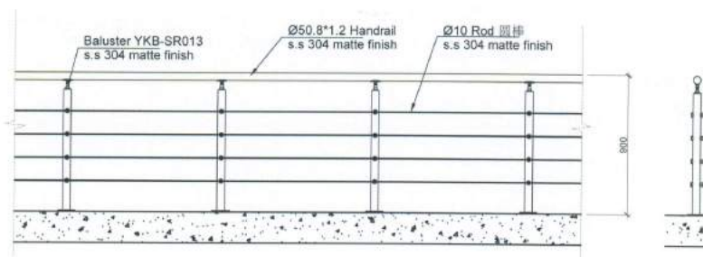
Railing Elevation 护栏立面图
