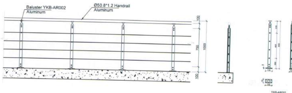
Railing Elevation 护栏立面图
