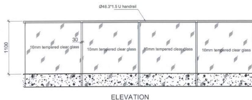
Railing Elevation 护栏立面图
