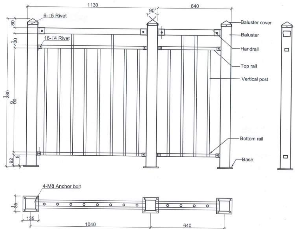
Railing Elevation 护栏立面图
