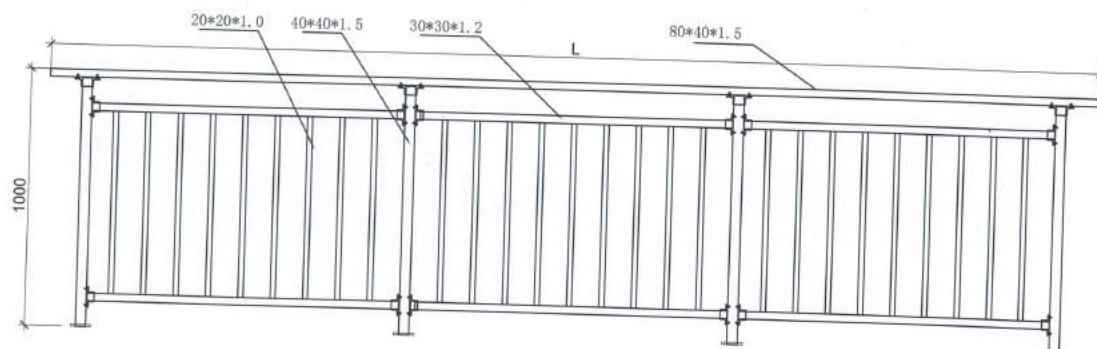
Railing Elevation 护栏立面图
