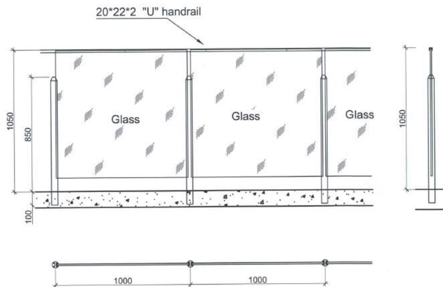
Railing Elevation 护栏立面图
