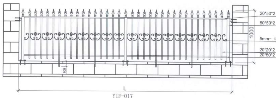
Railing Elevation 护栏立面图
