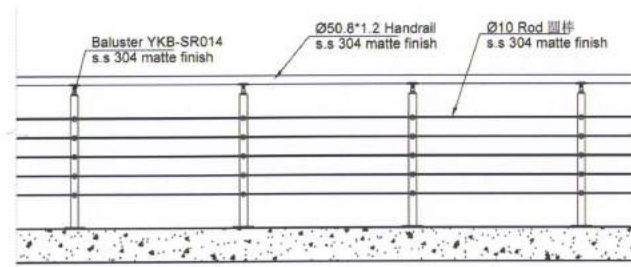
Railing Elevation 护栏立面图
