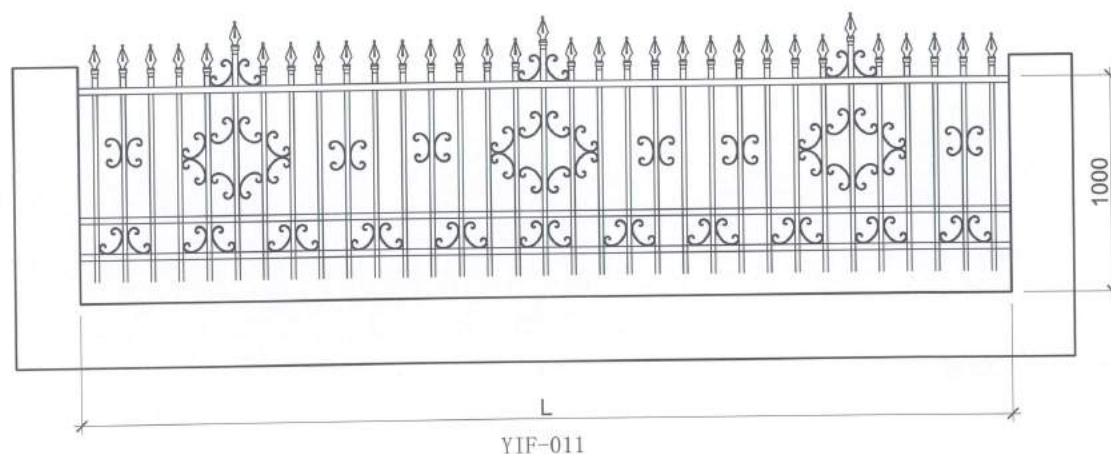
Railing Elevation 护栏立面图
