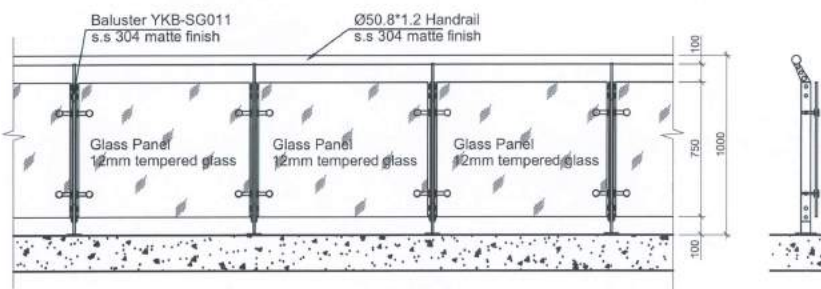
Railing Elevation 护栏立面图
