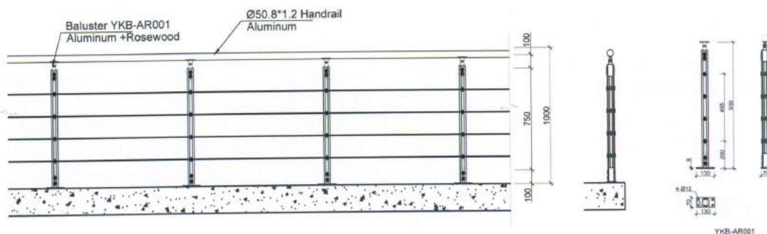
Railing Elevation 护栏立面图
