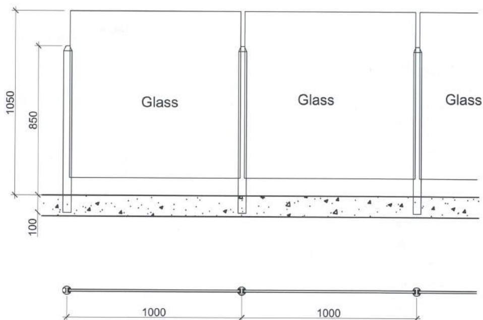
Railing Elevation 护栏立面图
